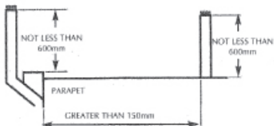
FLAT ROOF WITH PARAPET
