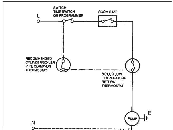
Fig. 6 Typical Wiring Diagram
