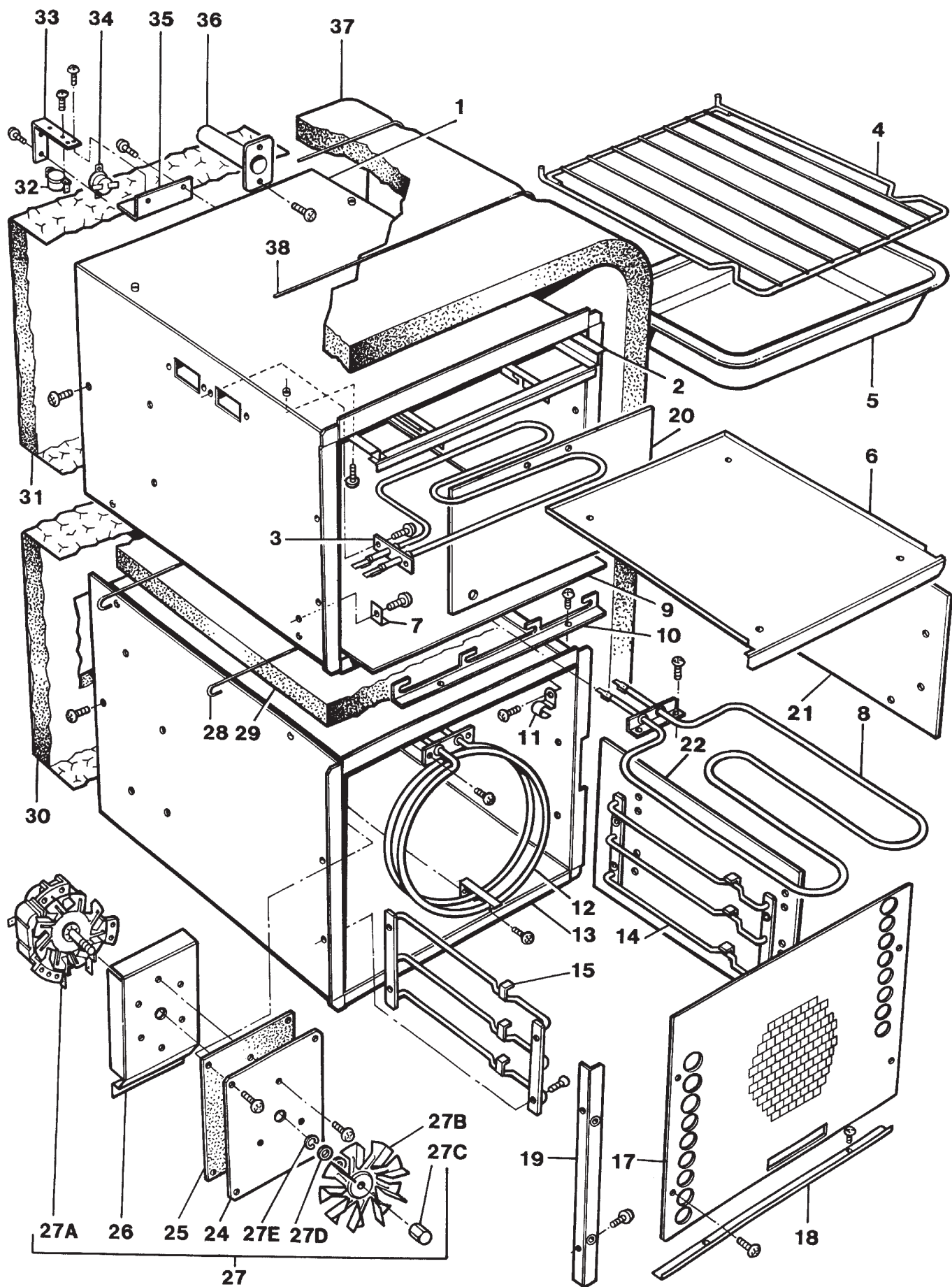
TOP & BOTTOM OVEN ASSEMBLIES AGA GAS MODULE
