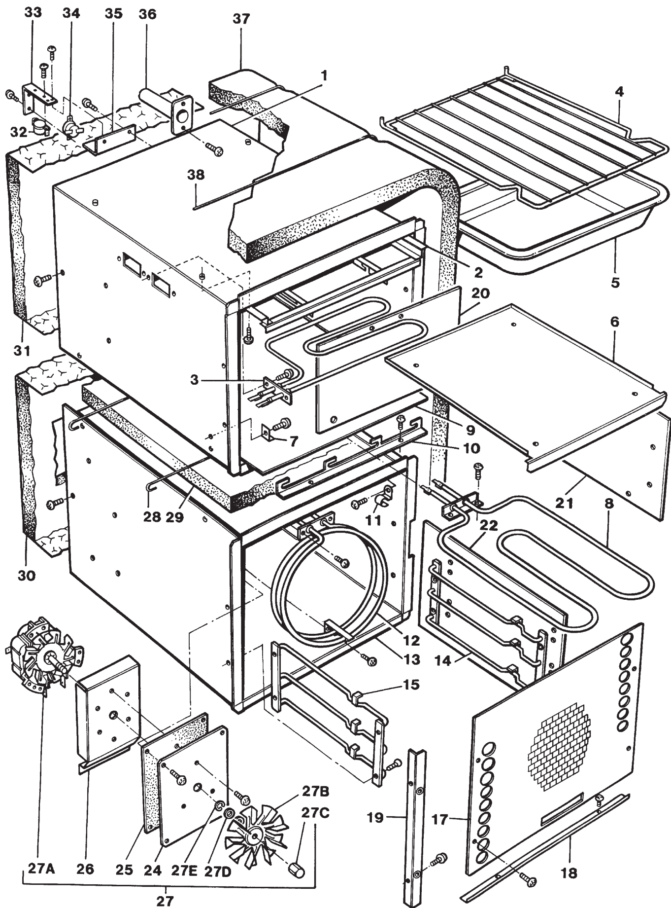
TOP & BOTTOM OVEN ASSEMBLIES AGA GAS MODULE NON FFD
