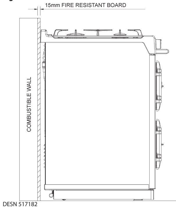
Fig. 12.3 COMBUSTIBLE WALL FITTING USING FIRE RESISTANT BOARD
