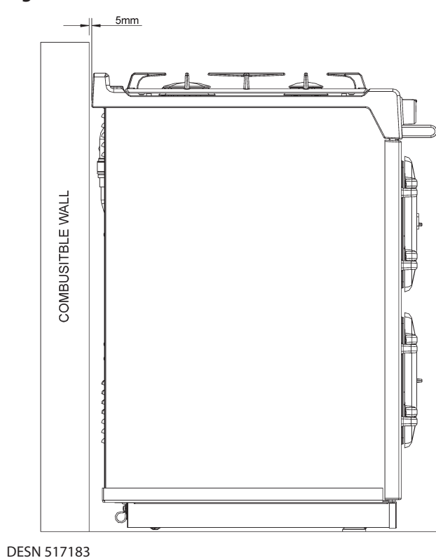
Fig. 12.4 COMBUSTIBLE WALL FITTING CLEARANCE
