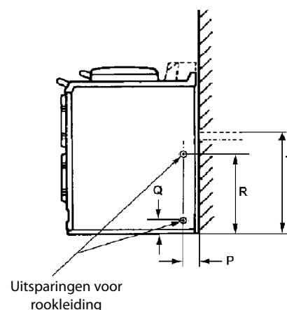
RH SIDE VIEW
